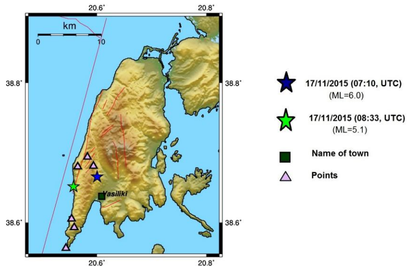
Figure 8. Map of Lefkada showing location of campaign GPS stations.
