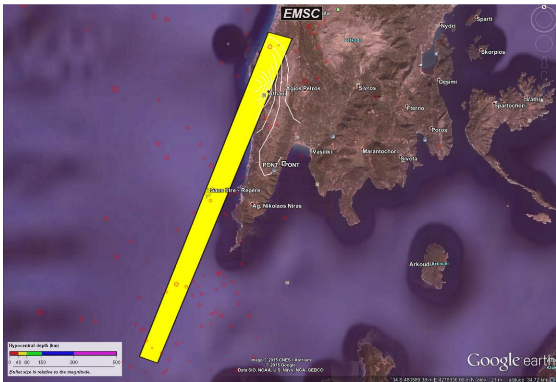
Figure 7. Preliminary fault model (yellow rectangle) of the Nov. 17 2015 event.
