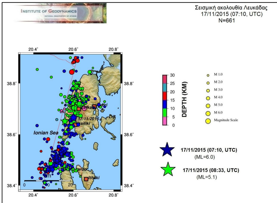
Figure 2 Seismicity map of the Lefkada sequence from NOA analysis (revised) data. Map contains 661 shallow events until Nov. 30th, 2015.
