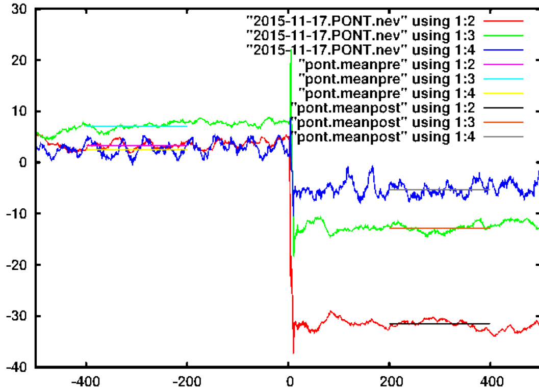
Figure 4. Graph showing static offsets of NOA station PONT (South Lefkada). Each time series shows the time window in which the average position (and the relative standard deviation) before and after the event have been computed. X-axis is time (s), Y-axis is displacement (cm).
