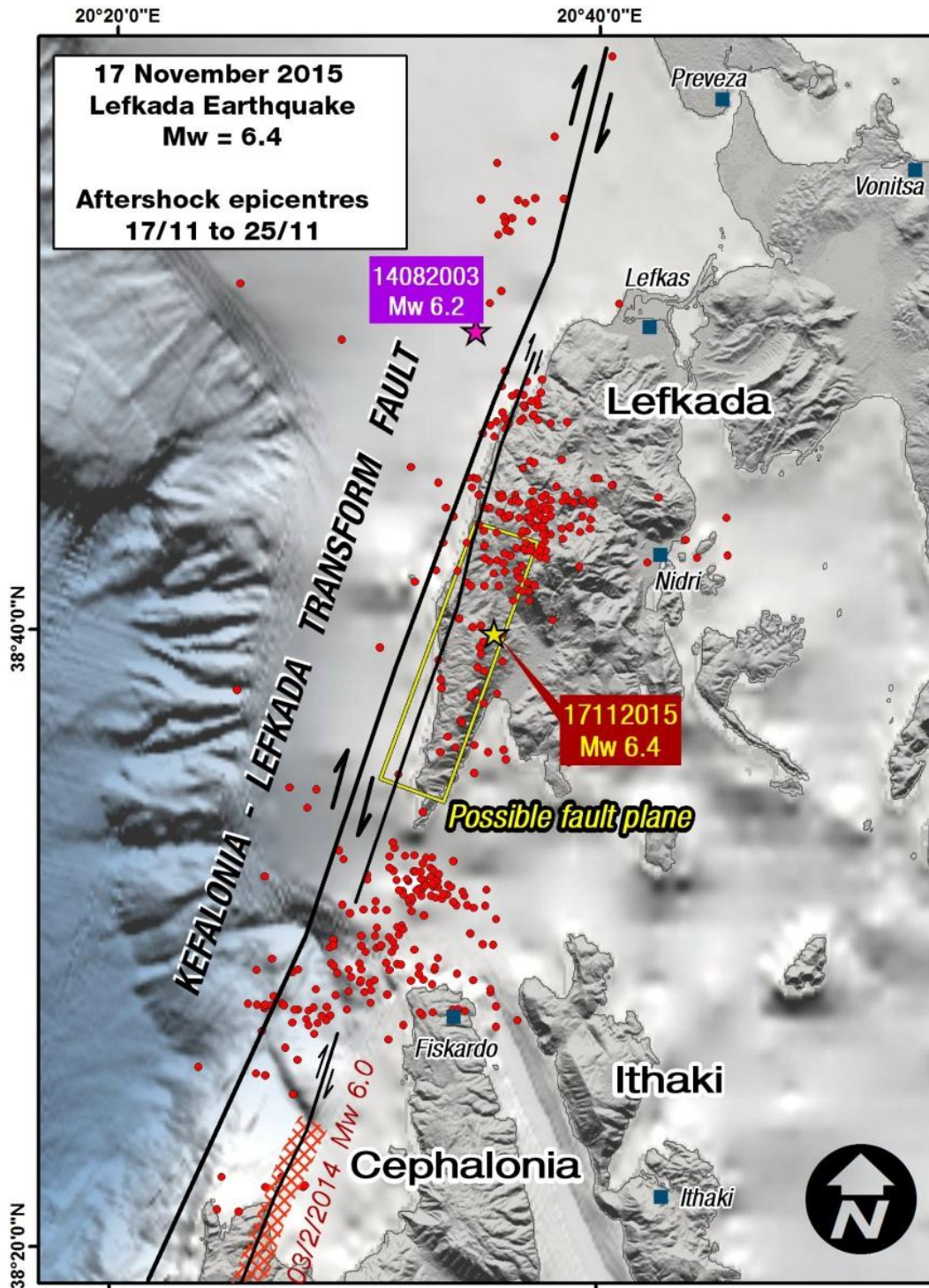
Figure 1. The 17th November 2015 Lefkada main earthquake (yellow star) and aftershock revised epicentres recorded by National Observatory of Athens (NOA). Dextral faults along the Cephalonia-Lefkada Transform boundary are shown as black lines.
