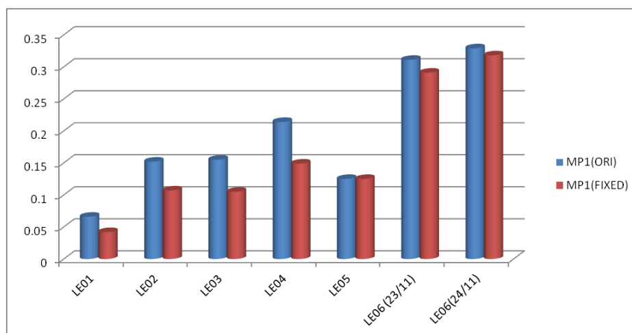
Figure 9. Excel chart showing L1 multipath suppression of six campaign stations in south Lefkada (November 2015 campaign).
