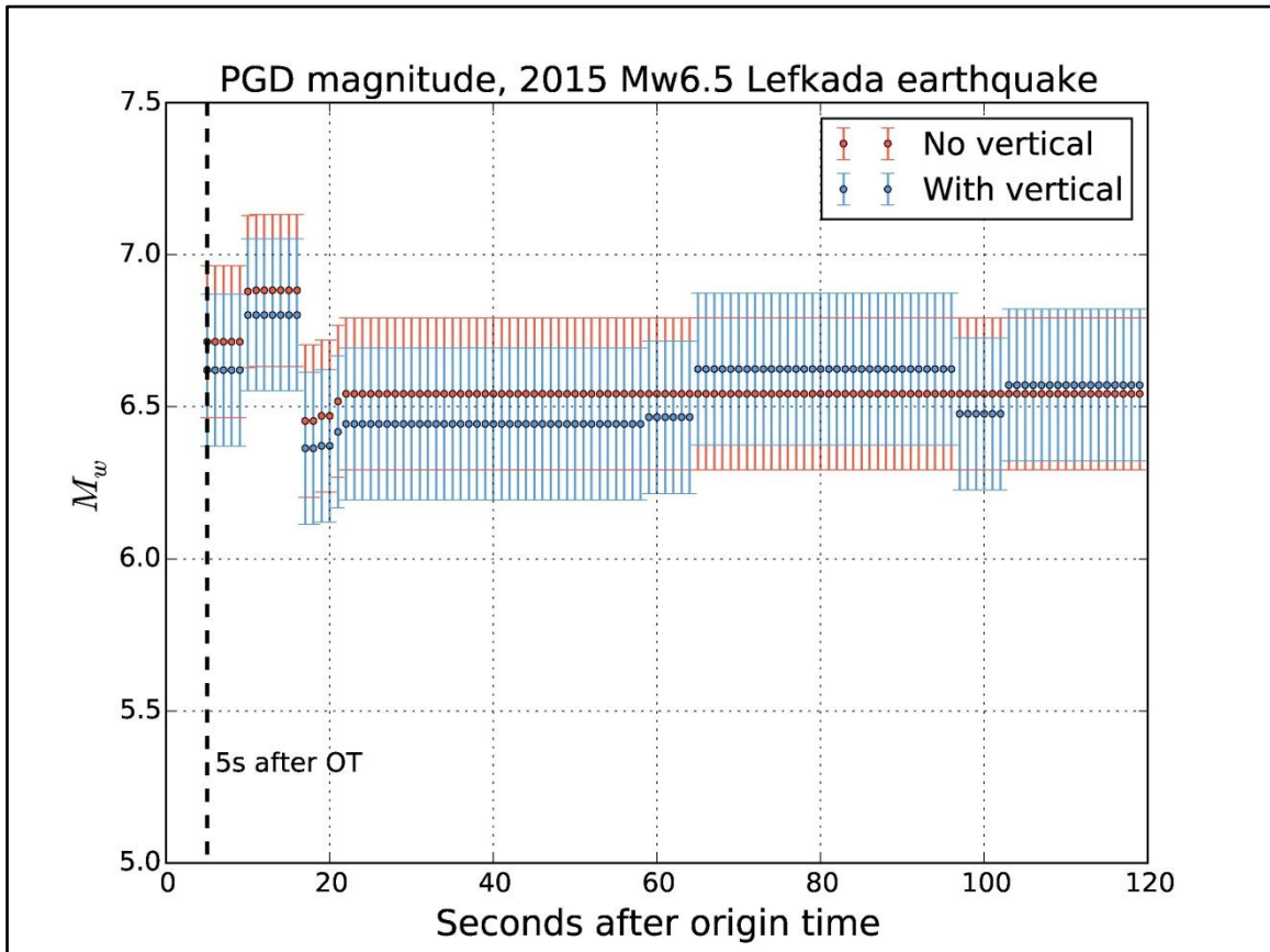
Figure 6. Plot showing the estimated moment magnitude ( M_w=6.5 ) from the high-rate GPS as a function of time with uncertainties. First estimate is at only 5s after origin time.
