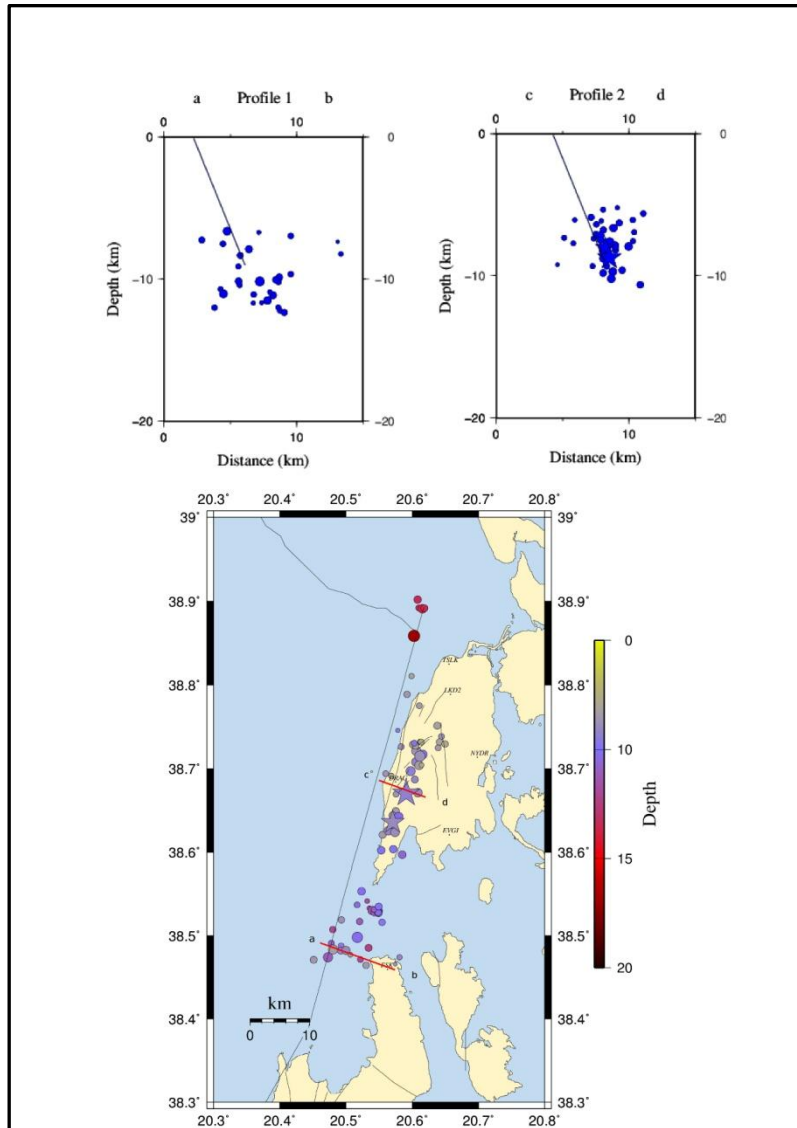
Figure 3. Map of relocated seismicity using NOA phase data (bottom) and E-W cross sections near the epicentre (top right; section c-d) and at the south end (top left; section a-b), respectively. Software used: NonLin-loc.
